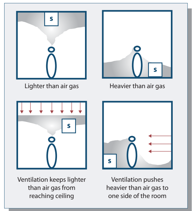
Sensor placement
